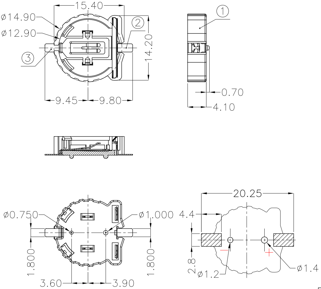
PCB Layout Diagram Top View
